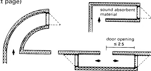
⑧ Plan of light and sound locks
